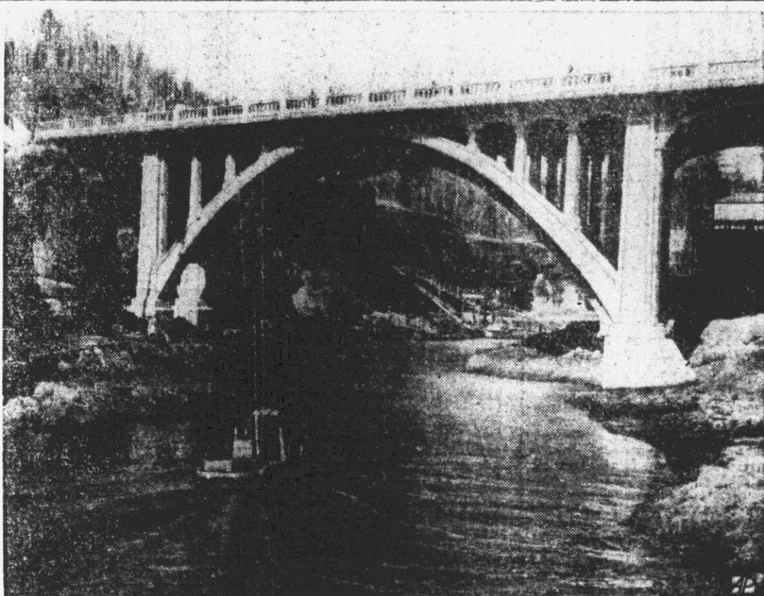
HEADACHE FOR MARINERS —A fishing boat makes its way through a harbor entrance believed the world's narrowest—22 feet wide, winding, and only nine feet deep—and leading from Pacific ocean to Depoe Bay, Ore. Only sports boats, fishing craft and trawlers can squeeze through. Overhead is the four-lane highway bridge of Oregon Coast highway, U.S. 101.
