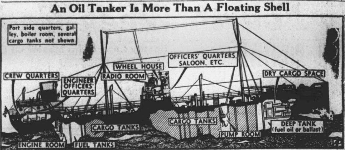
An Oil Tanker Is More Than A Floating Shell. A modern oil tanker is much more than a hollow shell. This cut-away drawing shows the major features of a new type of ship built for an American oil company. The catwalks above the low mid-sections are necessary because high waves sometimes break over the now decks. The need for more ships like this is a current defense problem.
