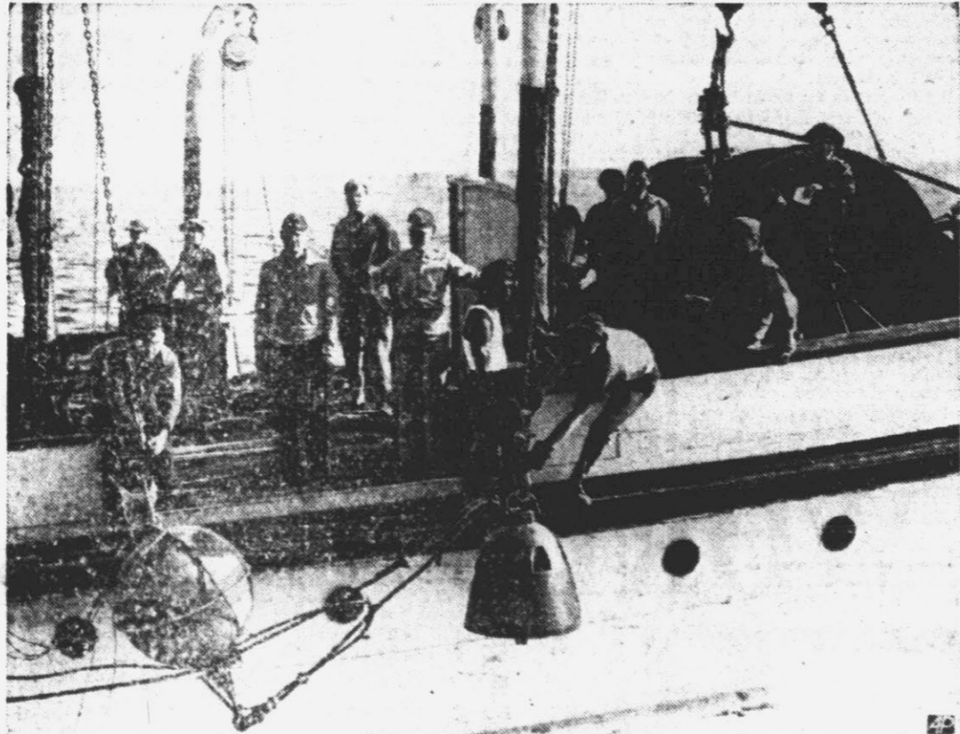
PLANTING SEASON FOR MINES —Soldiers of the 5th and 7th coast artillery regiments lower a mine and its anchor into the waters off Sandy Hook Point, outside the entrance to New York harbor. This practice in mine-laying will continue until September. The mines can be exploded from shore or, after adjustment, by contact with a ship. Mines have reduced charges.
