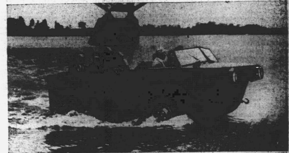
AMPHIBIAN WITH AMBITION —With an eye on possible acceptance as a scout car by the U.S. army, this amphibian invented by Roger W. Hofheins of Buffalo tackled the swift Niagara river for its tests. The four wheels and three-bladed propeller are powered by a regular auto motor, each wheel being hinged to the body and driven by a chain. It can carry 20 persons.
