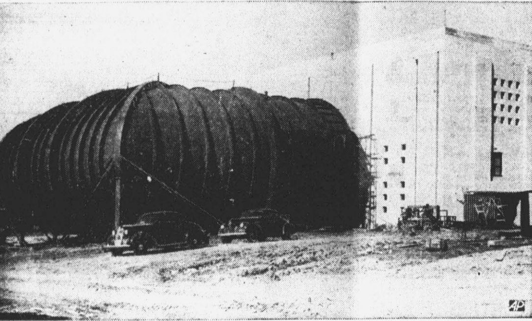
LOOK OUT FOR THE BIG WIND —Almost completed at Wright Field near Dayton, Ohio, is the army air corps experimental station's new $2,500,000 wind tunnel, where a 50,000-horsepower electric motor will produce wind velocities up to about 400 m.p.h. The tunnel, 790 feet long, will accommodate a model plane with 15-foot wingspread. Tunnel was begun year and half ago.
