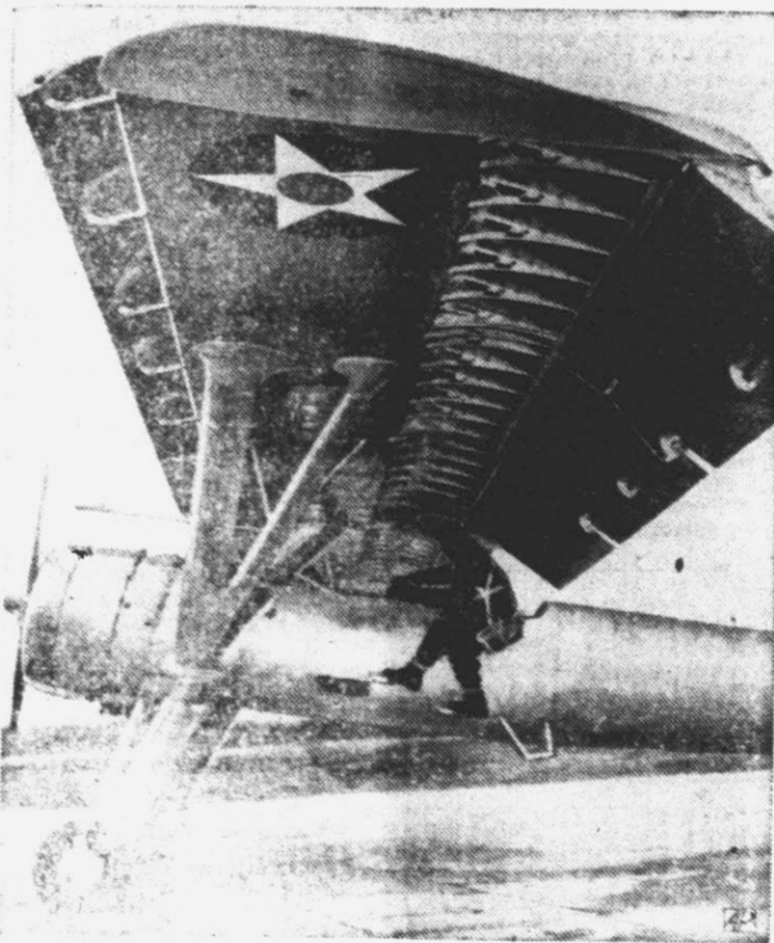
ARMY JEEP —Testing this plane at Fort Benning, Ga., is the "Jeep" flying slots on the leading edge and wide flaps on the trailing edge allow for quick takeoffs and landings at 25 m.p.h. Plane may serve as a courier.
