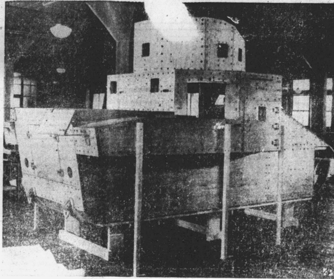
TANK—IN THE ROUGH! —Chrysler engineers, working on a defense order for U.S. army tanks, to be built outside Detroit in a new tank plant, made this preliminary wooden work-up model which is, however, not the model from which the tanks are to be built. Some 5,000 persons probably will be working by late summer producing five 25-ton tanks in one shift per day at the plant.
