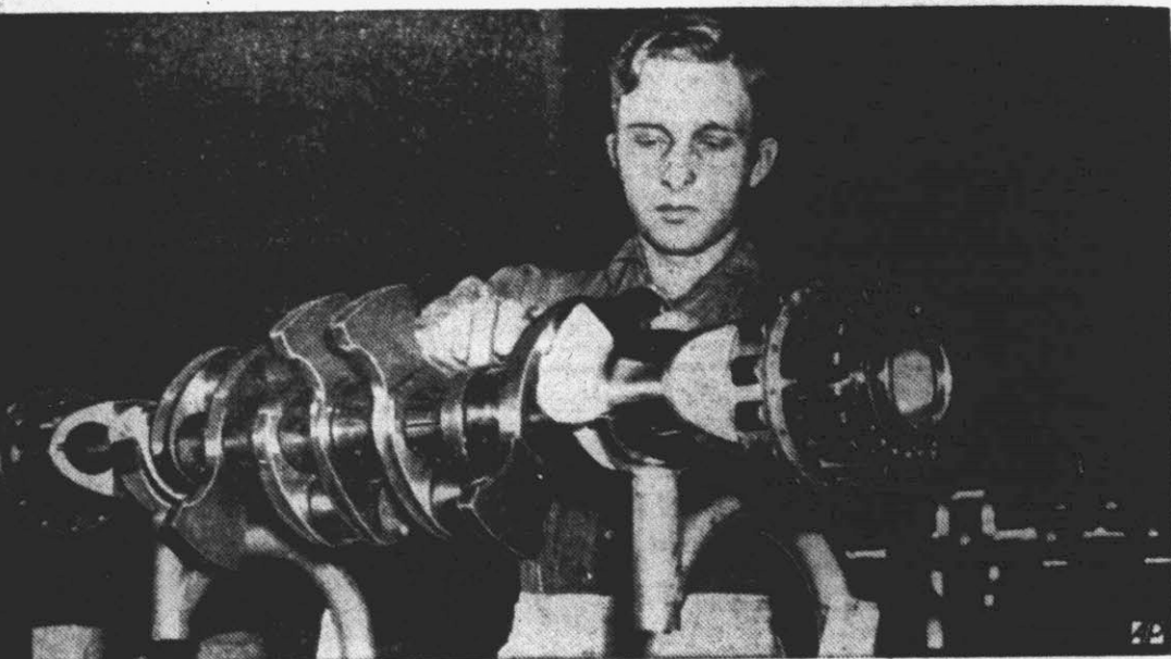
PART OF PLANE'S POWER —Close-up shows build of crankshaft that takes the pounding of 12 cylinders in Allison plane engines being turned out at rate of 350 a month in Indianapolis.
