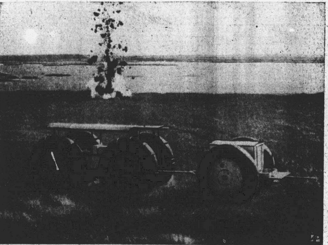
MONSTER OF THE MARSHES —With this marsh buggy and trailer, scientists have been exploring Louisiana marshes in search of "black gold." The trailer carries geological instruments used to record the man-produced explosions such as that in the rear. Blasts of dynamite shake the earth, and from these recordings engineers determine where to drill for oil.
