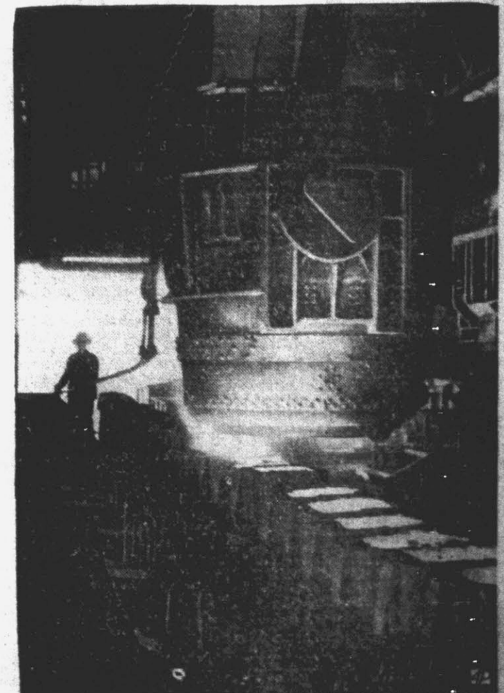
STEEL MILLS BOOM —Here's a pit scene in the open hearth plant of the Tennessee Coal, Iron and Railroad Co. near Birmingham, Ala., as steel is teemed into ingot molds. Countless big orders have boomed steel mill activity.
