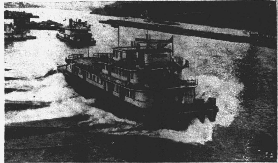
EVEN THE RIVER FEELS NAVAL BOOM —Here's the William Penn, one of the largest motorships built for river freight traffic, as she slipped down ways at Pittsburgh. It was built for operation on the Mississippi and Ohio rivers. The Diesel-powered towboat, 176 feet long, will push and flank barge flotillas carrying some 10,000 tons of freight.
