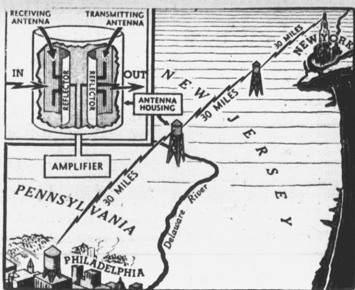
Map of proposed circuit (New York to Philadelphia) of the world's first ultra-short-wave television network. Positions of relay stations are approximate.
