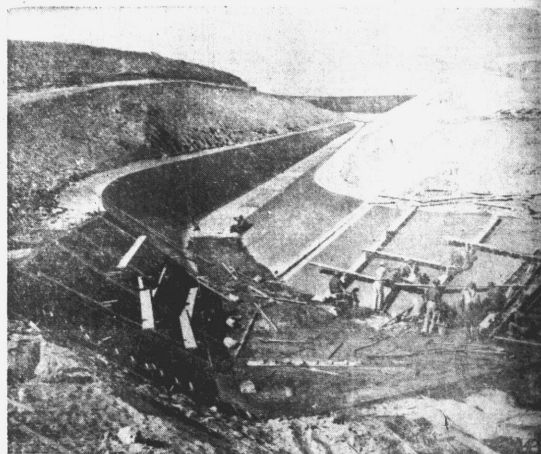
EVERYTHING'S ROZA OUT YAKIMA WAY —First delivery of water through the Yakima Ridge canal (above) in Washington is scheduled for 1941, according to Bureau of Reclamation engineers building the Roza diversion dam in the Yakima river. Above view shows the transition from a concrete lined section to an earth section of the canal. Some 72,000 acres will be watered.
