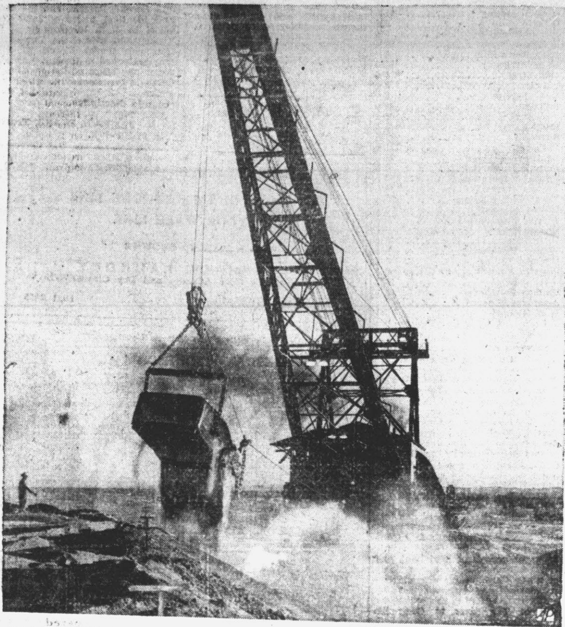
MAN POWER BOWS TO MACHINE —Thirty-two tons of sand at a bite are lifted by this giant shovel, now digging a 134-mile addition to the All-American canal from the Colorado river to California's Imperial valley. The addition, called Coachella branch, will carry water to the Coachella valley, making possible the irrigation of 137,000 acres of rich desert land.
