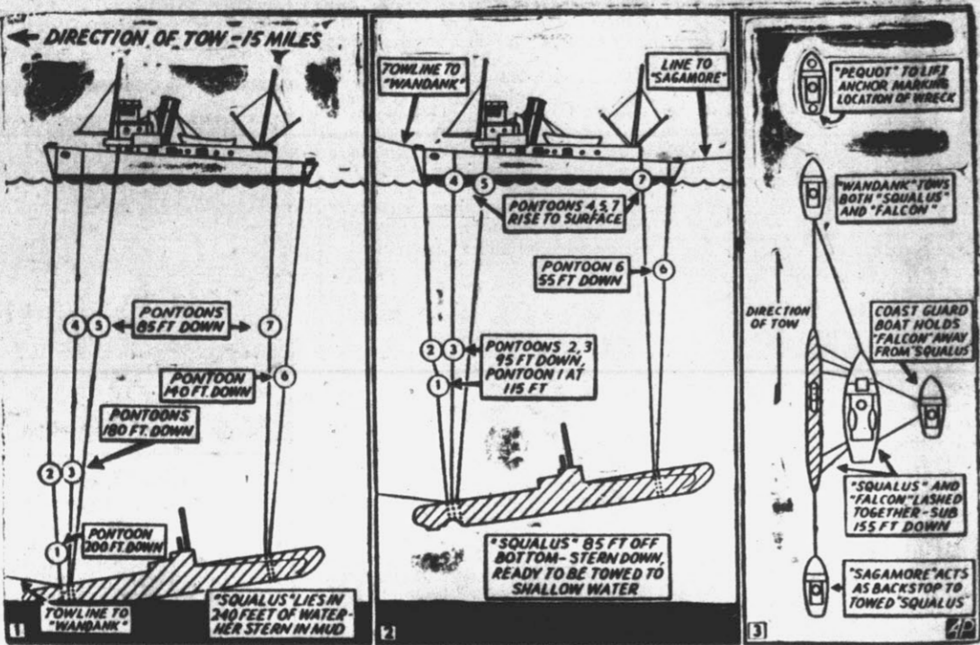
This chart shows the methods by which navy men hope to lift the sunken submarine Squalus off Portsmouth, N. H., and tow her to shore by gradual stages. Seven pontoons are being used. With only two yet to be attached, the first lift is expected to be made July 12. The drawing at the left shows how the pontoons will be placed. In the center are the three pontoons designed to rise to the surface. The illustration at the right shows the manner in which the towing unit will function with vessels assisting the salvage ship Falcon in keeping tow d submarine under control. The Squalus sank May 23.
