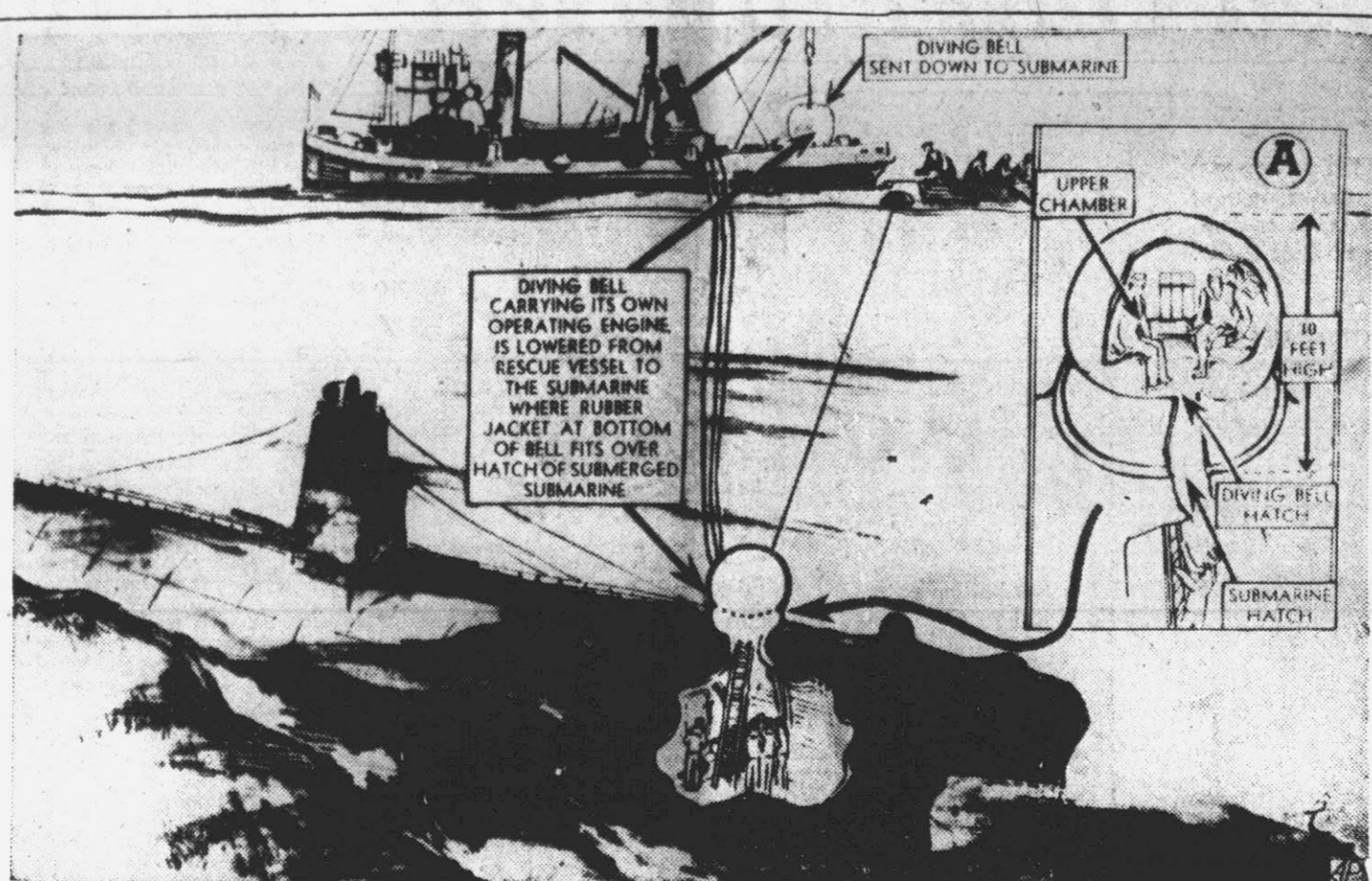
This drawing shows how the rescue ship Falcon saved survivors of the sunken submarine Squalus with a huge diving bell off Portsmouth, N. H. The bell is shown fitted over the hatch of the stricken vessel for the men to enter it and be raised to the surface. Inset A represents an enlargement of the bell which can hold six to eight men. Twenty-six of the Squalus' crew were believed dead.—(Associated Press Photo from The Chicago Tribune.)
