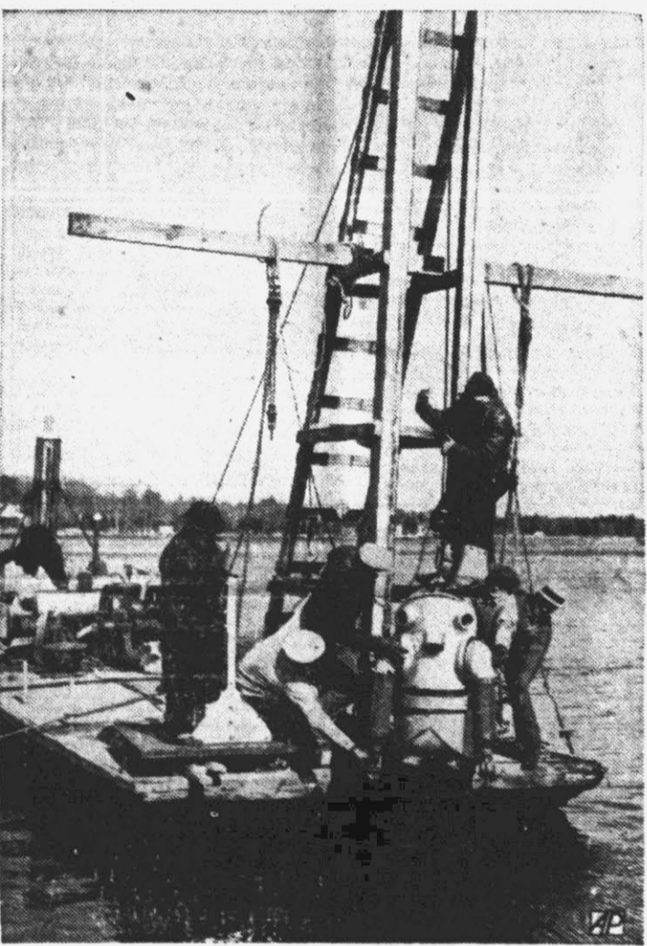
STARTING AT THE TOP and working down, Cyril von Baumann (inside the suit) tests a new diving outfit at Toms River, N. J. The suit, which has a total weight of 1,100 pounds, was designed by Capt. Tom Connelly, and is lowered into the water by means of a marine derrick. Oxygen and helium are combined—for the first time, it is thought—in this type suit.
