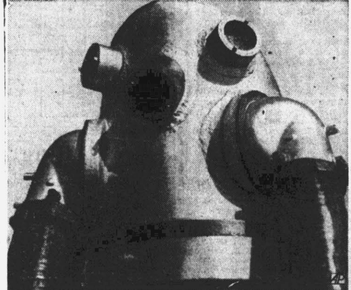
TO SEE THE SEA at depths not previously reached by divers, Capt. Tom Connelly of Jersey City designed this diving suit, recently tested by Cyril von Baumann at Toms River, N. J. The suit, in which a combination of oxygen and helium is used, is a self-contained unit made of cast manganese bronze covered with sheet chromium steel. It claims unofficial tests at 571 feet.
