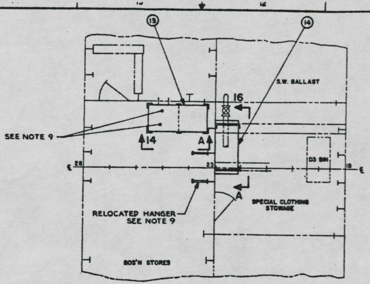
PLAN AT BOS'N STORES LCU 1667-1670 ONLY
