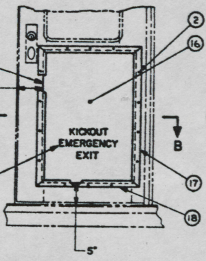
VIEW 11-A SCALE NONE KICK-OUT PANEL IN W.R.-S.R.
