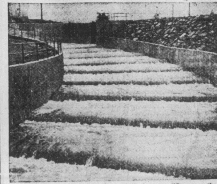
SO THE U. S. government provided ladders like this one so the salmon could get around the dam. Each step of the ladder is two feet high.
