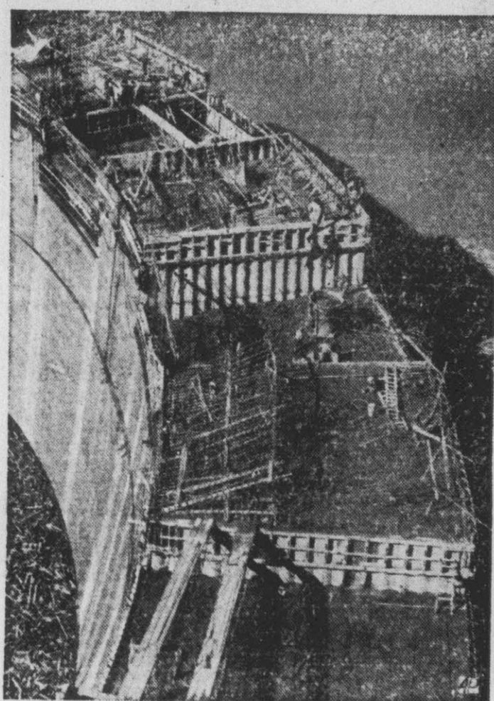
CORRUGATED EDGE of interlocking forms is an architectural note at Parker dam on Colorado river 150 miles below Boulder dam. Concrete is now being poured.
