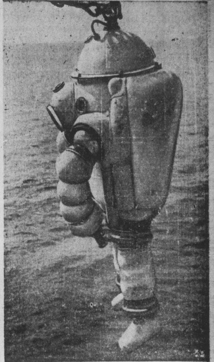
NOT 'DOPEY,' THE DWARF , this is a new diving apparatus at La Spezia on the west coast of Italy by G. Galeazzi, who's giving it tests in the Gulf of Genoa. The diving apparatus, which weighs almost 900 pounds, went down to a depth of about 800 feet on its preliminary trials at La Spezia.
