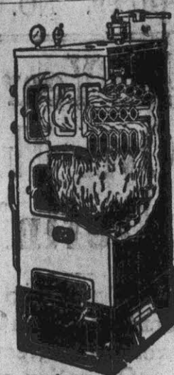
Cutaway view of the popular No. 2 National Jacketed Boiler—one of the 150 sizes and types.
