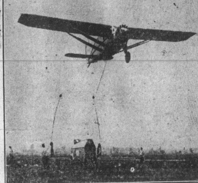
Demonstrating the new Cabot aerial pickup at Roosevelt field, N. Y. Mail bags fastened to long poles with a cord between them are picked up by a plane going at full speed. A pole with a hook extending below the plane picks up the bags which are then pulled up into the ship.
