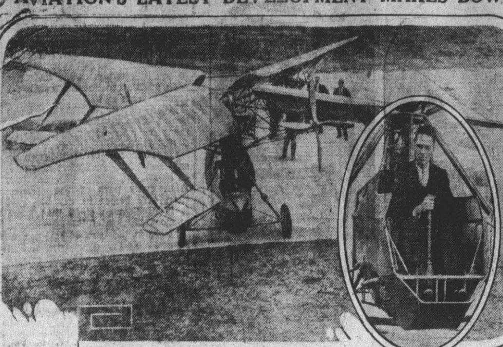
The helicopter, designed to meet the need for an airplane that will move directly up and down, received initial tests at Curtiss field, New York. The craft consists, essentially, of four large wings or blades made to revolve by propellers mounted on each wing and receiving their power from a centrally located motor. Maitland B. Blecker, the inventor, is shown in inset at the controls of the new machine.
