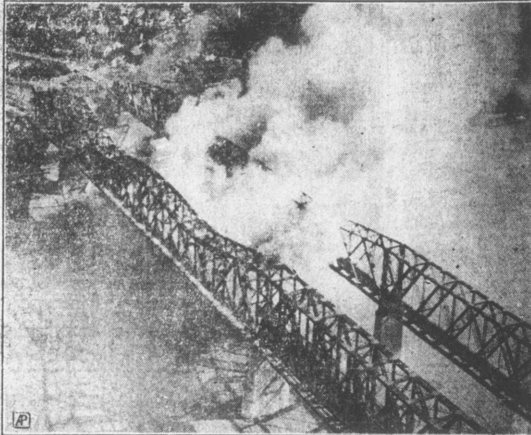
Vehicular traffic between Memphis and Arkansas was paralyzed when fire destroyed a large section of the wooden floor work of the $4,000,000 Harahan bridge over the Mississippi river. Hundreds of automobiles on both sides of the river were caught behind the blaze.
