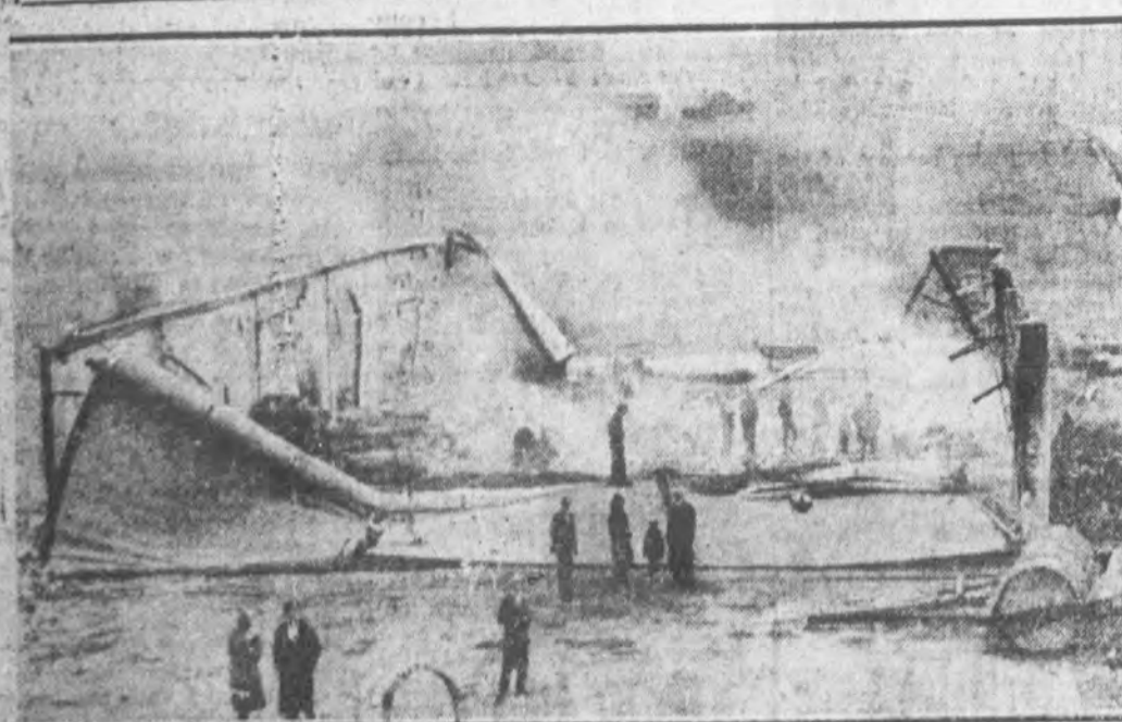
This shows the ruins of the Colonial Air Line hangar at New Brunswick, N. J., where fire, started by an explosion of a heater, destroyed five Sikorsky airplanes, tying up temporarily the New York and Boston air mail. Five motor trucks and twenty motors were also destroyed, bringing the damage toll to $250,000.
