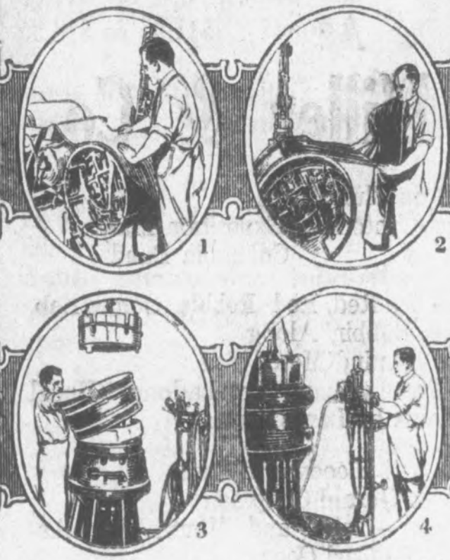
Steps in Building a United States Tire by the Flat Band Method
