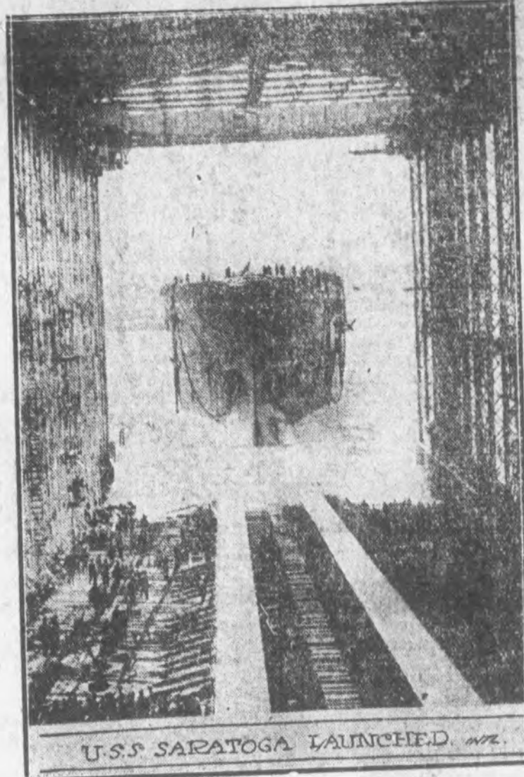
Above is shown the U. S. S. Saratoga, largest and speediest airplane carrier in the world, gliding into the water from the ways at Camden, N. J., after she had been christened by Mrs. Curtis D. Wilbur, wife of the Secretary of the Navy. The 33,000-ton ship, with a speed of thirty-nine land miles an hour, will cost $45,000,000 when completed. She will carry seventy-two airplanes, which she launches from her flat decks.
