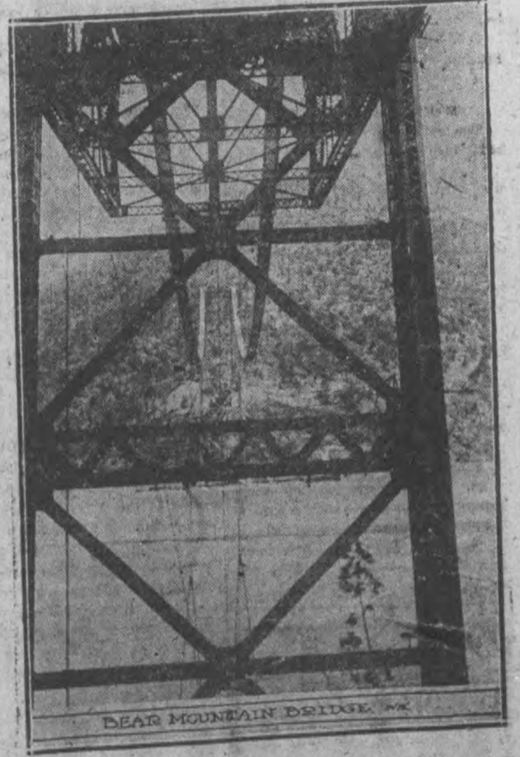
Tiny foot bridges have been swung from the world's largest suspended bridge, which is being built across the mighty Hudson River at Bear Mountain, New York State's great playground. The foot bridges are suspended from towers 365 feet high. The bridge is 1,632 feet long between towers and is just above Peekskill, N. Y. It will be completed in 1925 for foot and vehicular traffic.
