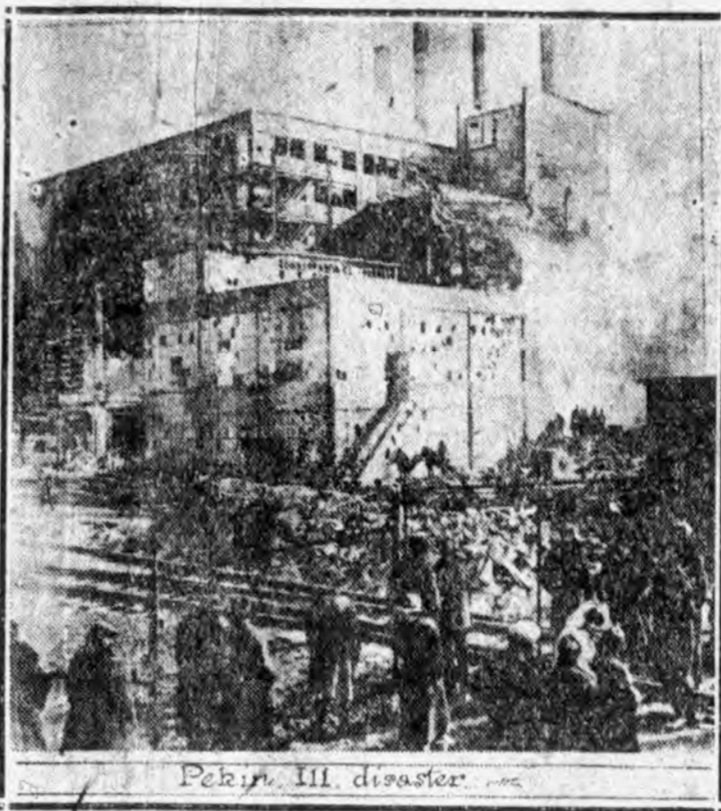
This photograph shows one of the buildings of the Corn Products Company, at Pekin, Ill., after a dust explosion and fire which wrecked two buildings of the immense plant, killing more than 30 and injuring a large number. Note how completely the structure was wrecked.
