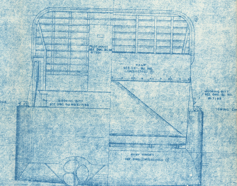
STERN VIEW
