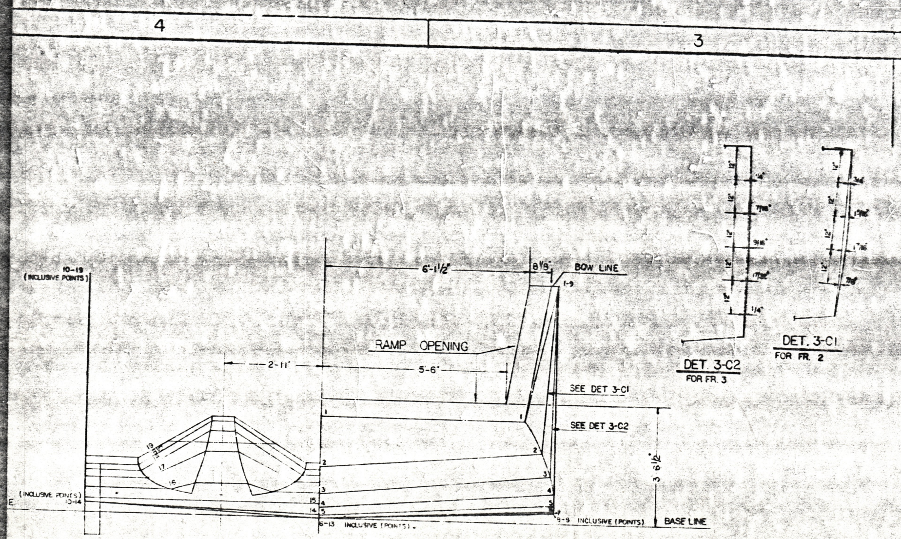
BODY PLAN FOR LINED PREG. REFER TO DWG NO 114 5033173
