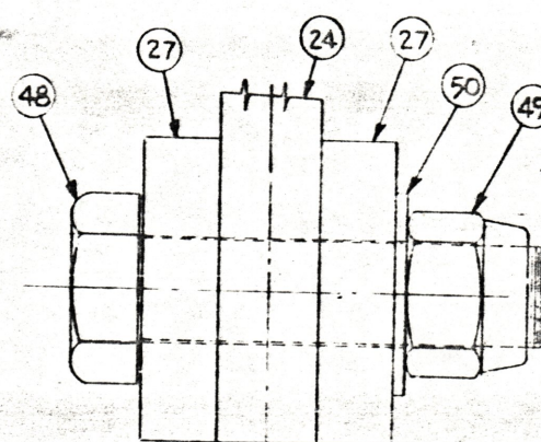
DETAIL 7-D PINTLE SUPPORT ASSEMBLY ITEM 26 & 23 OMITTED FOR CLARITY SCALE: 1/1 (8A)
