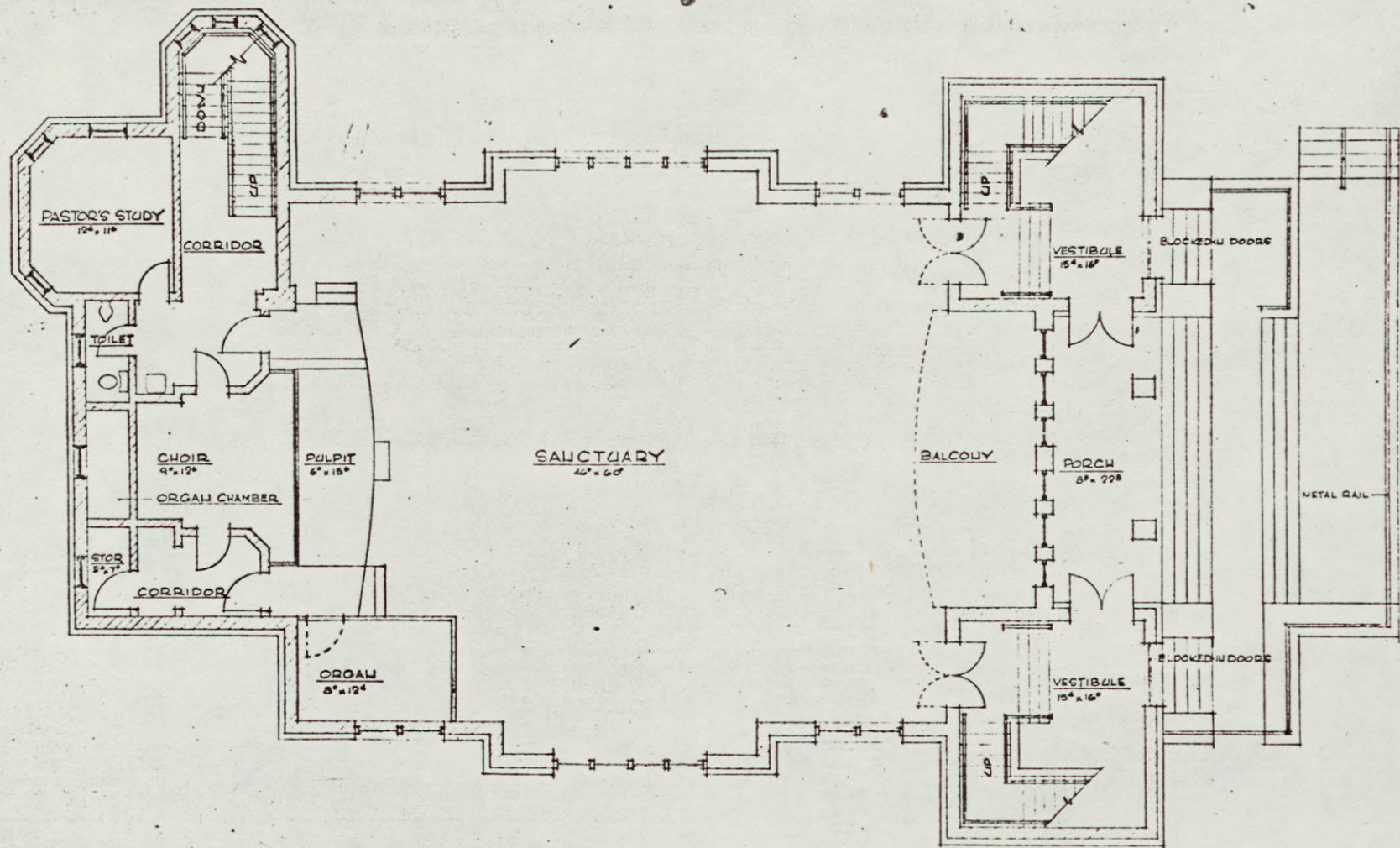
FIRST FLOOR PLAN SCALE 1/4" = 1'-0"
