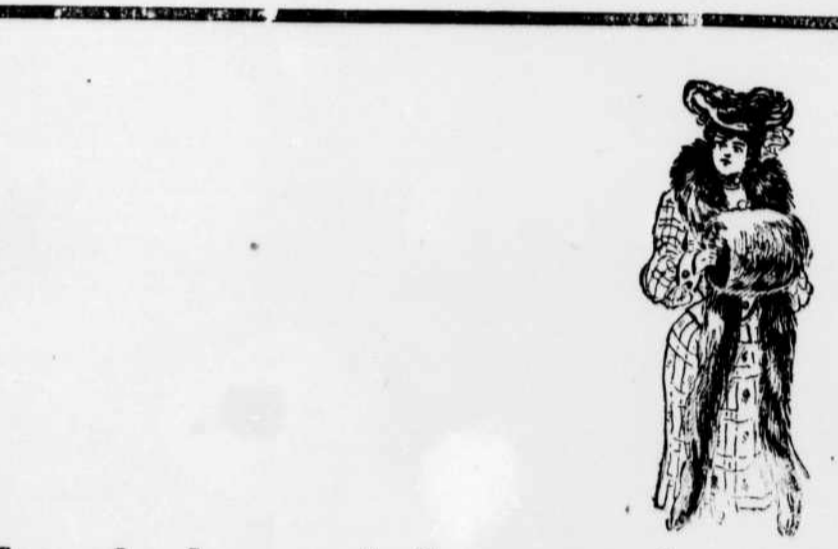
Dorothy Dodd
