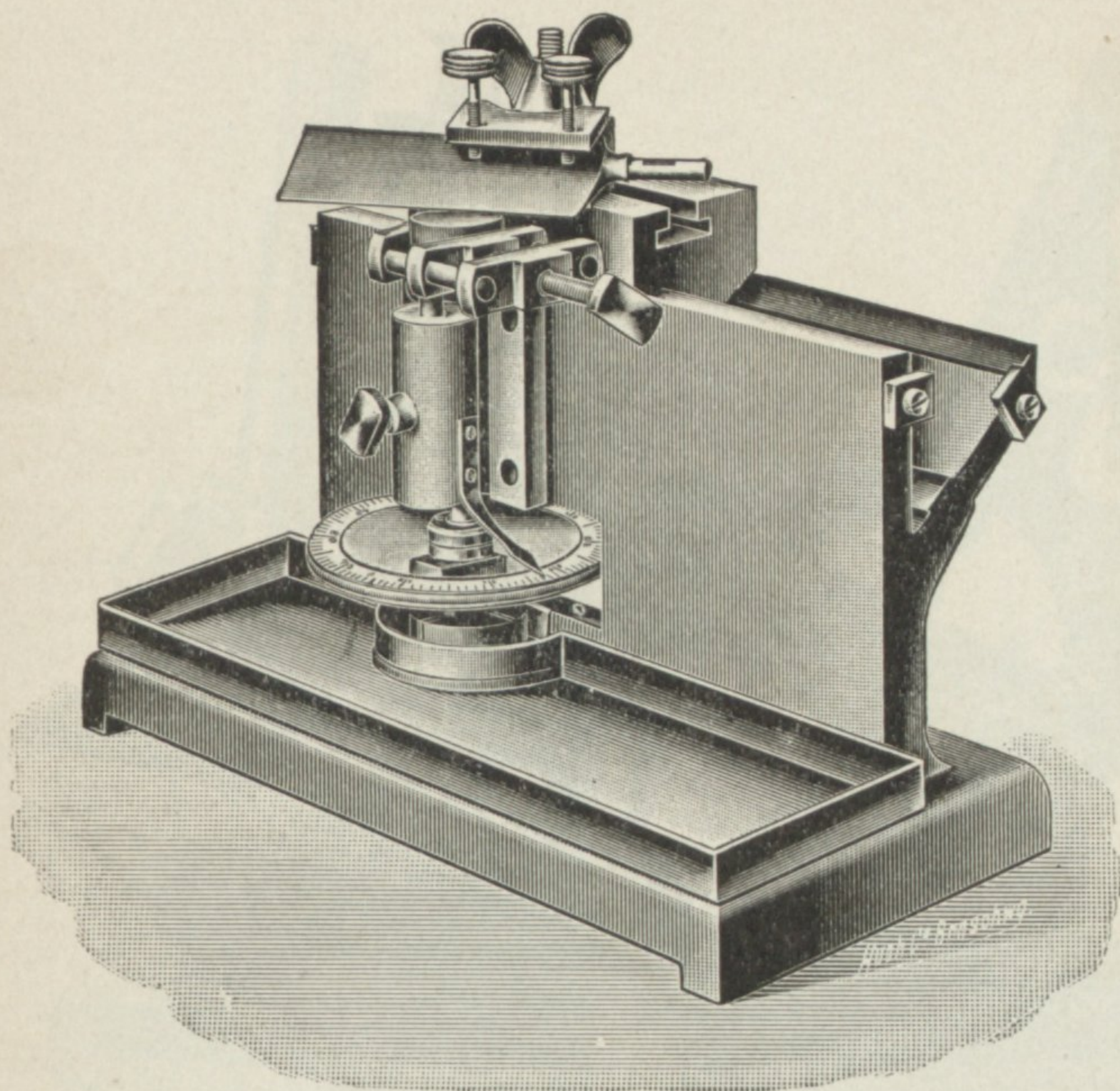
SLIDING MICROTOME T/.187.
