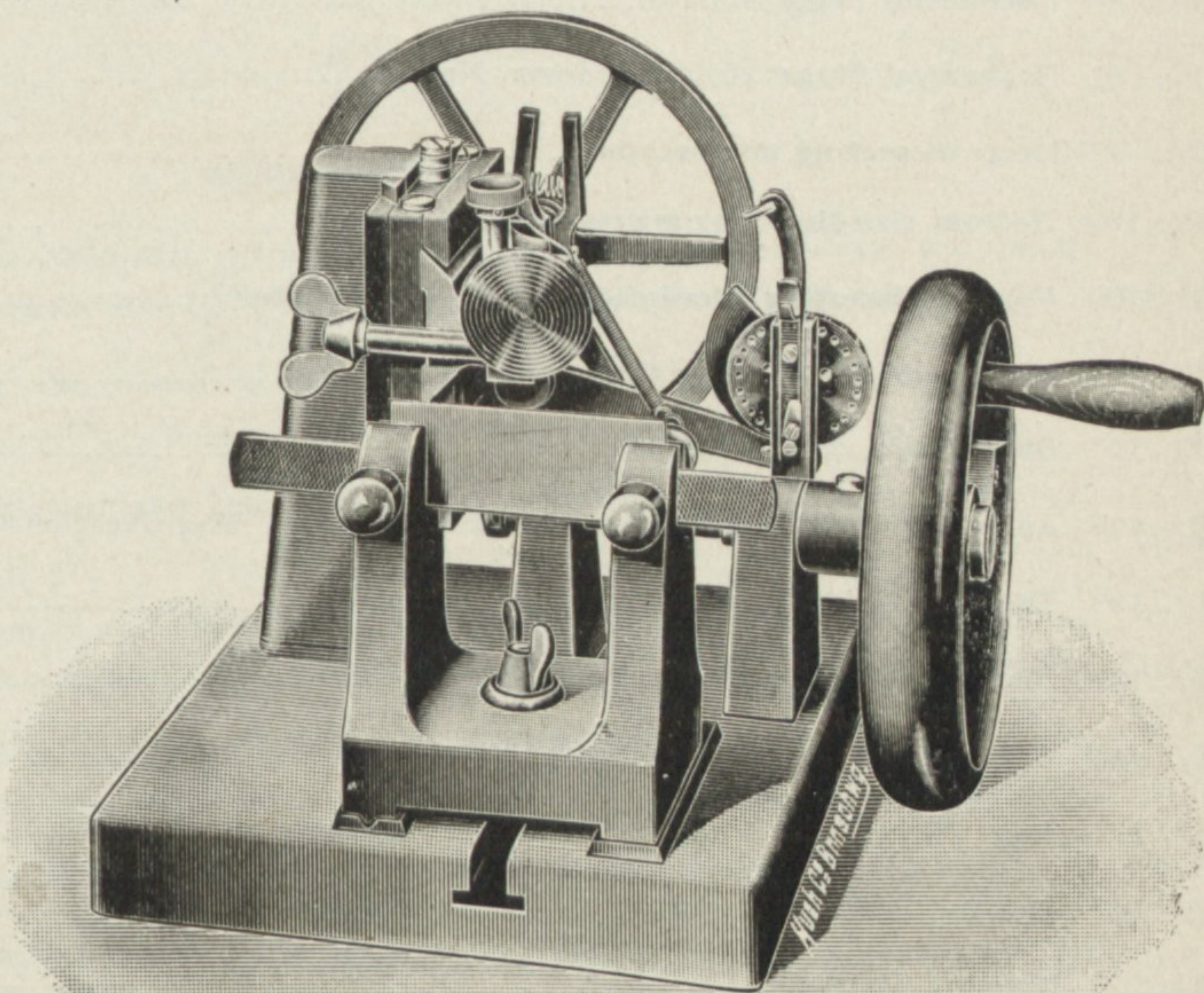
SLIDING MICROTOME T/.187.
