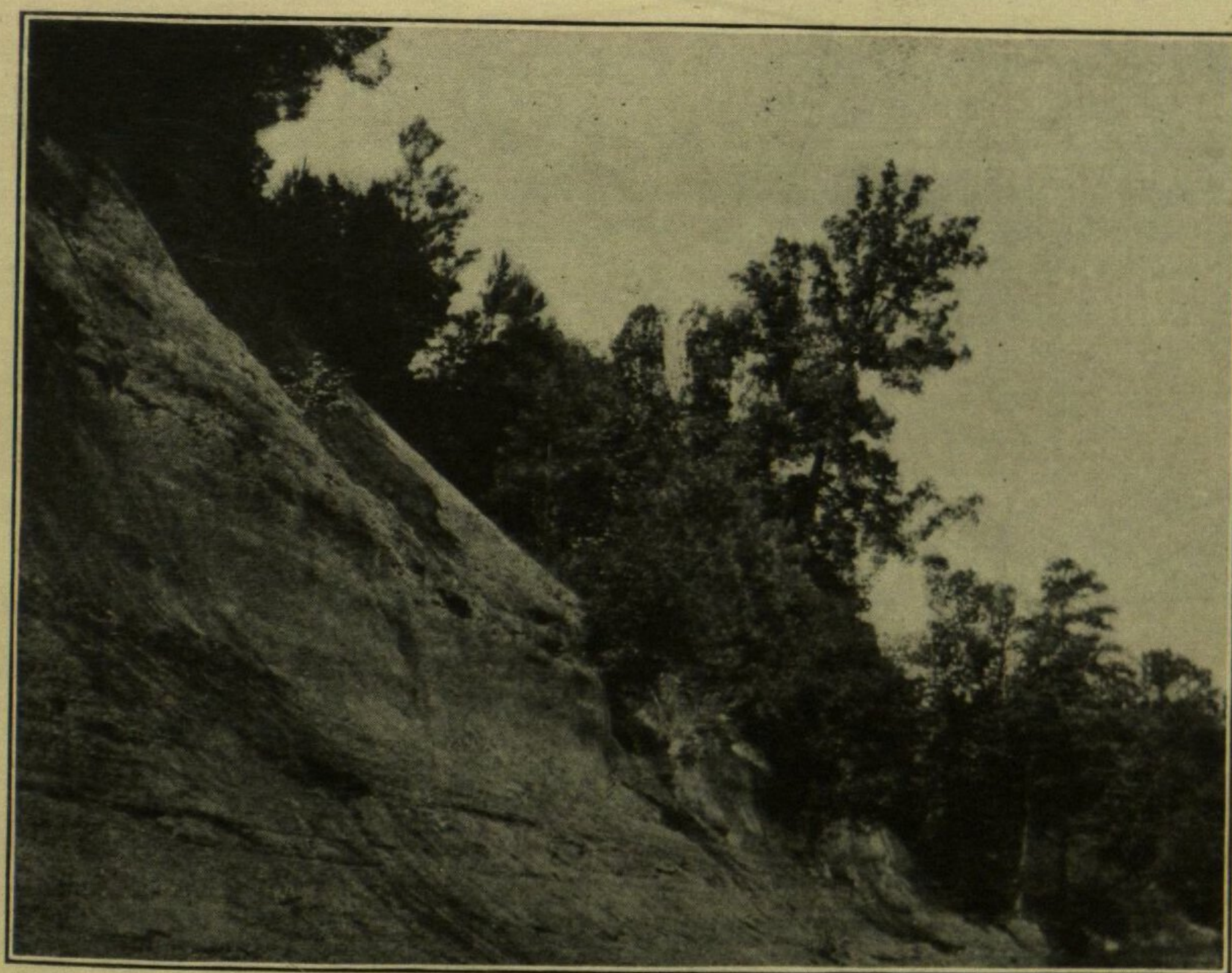
B.—Bluff at Blue Banks Landing, Tar River, seven miles above Greenville, N. C., showing the Black Creek formation overlain by the St. Marys formation.
