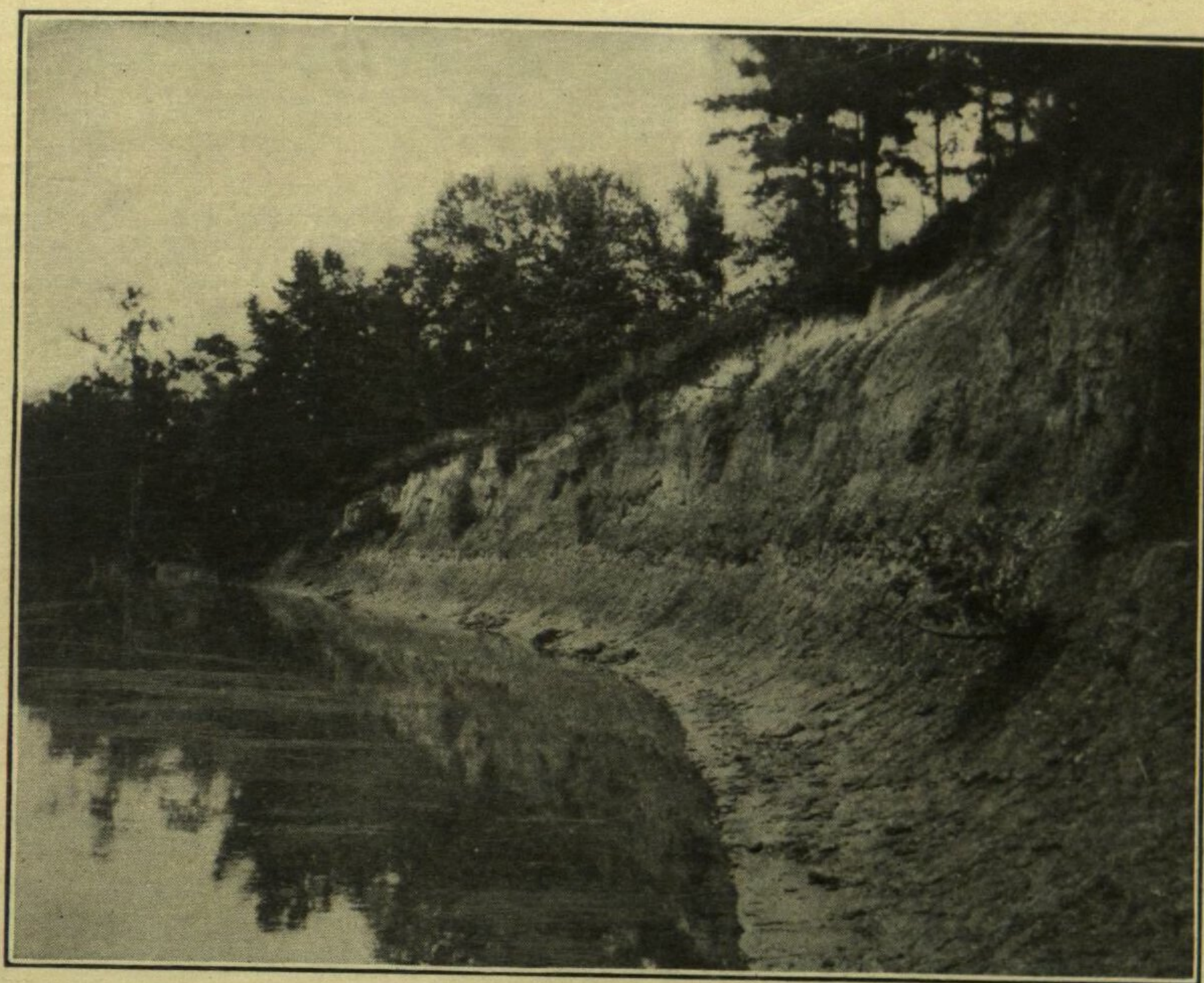
A.—Exposure showing the Patuxent formation overlain unconformably by the St. Marys formation, and the latter in turn overlain by Pleistocene deposits, Roanoke River, one mile above the State Farm, Halifax County, N. C.
