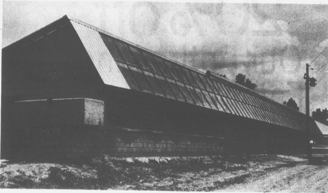
CATCHING SOME RAYS — The 51 solar panel collectors on the roof of Don and Ann Wilcox's self-contained feeder pig operation will help provide approximately two-thirds of the building's heating needs during the year. Pork producers from across
