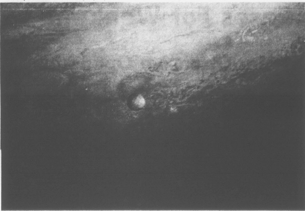
ANOTHER LOOK AT JUPITER — This photo of the southern hemisphere of Jupiter was taken by Voyager II on June 25, 1979 at a distance of 8 million
