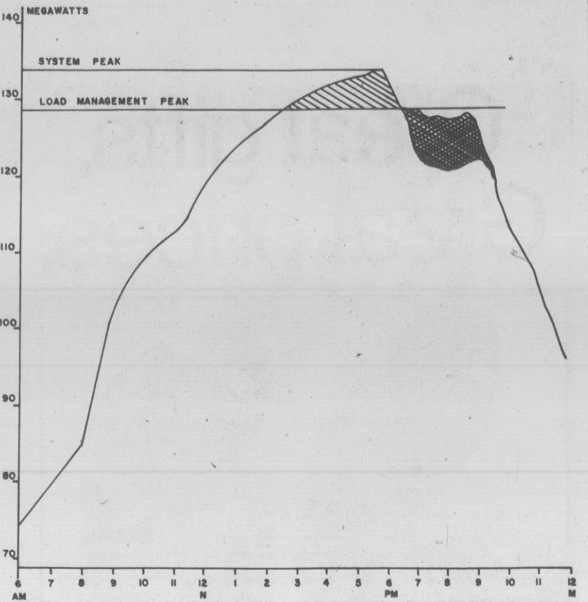
"BEAT THE PEAK" — This graph provided by the Greenville Utilities Commission illustrates the five megawatt demand reduction programmed for the commission's load management program. The 5 mw peak at the top of the graph would be shaved
