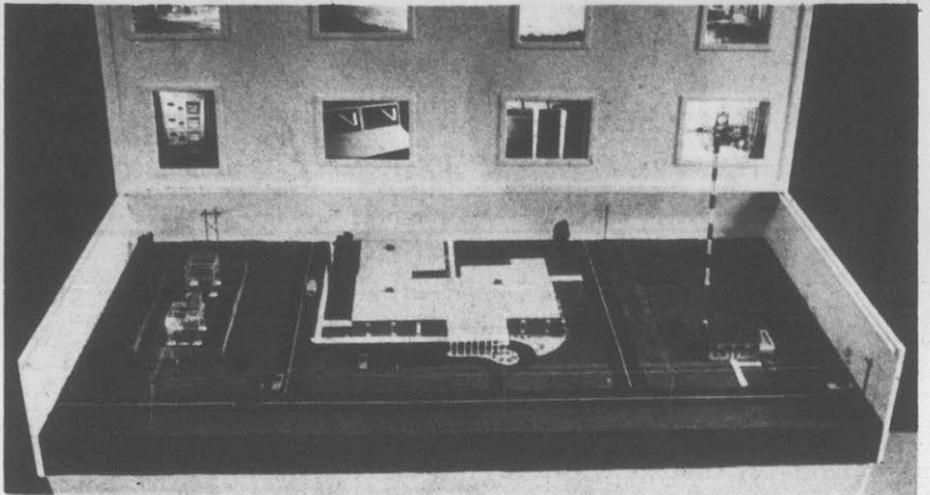
MODEL SYSTEM — This model illustrates how GUC's load management program will work. Telemetry signals will be sent from the power sub-station at left to the "Beat The Peak" center where programmers will pick up the signals. Radio transmitters
