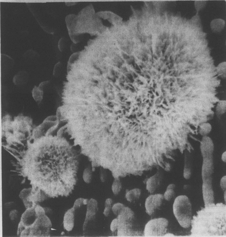
DANDY LYING —What appear to be dandelions gone to seed are actually iron oxide crystals that grew on a fireback from a high-temperature laboratory furnace. They are magnified 6,000
