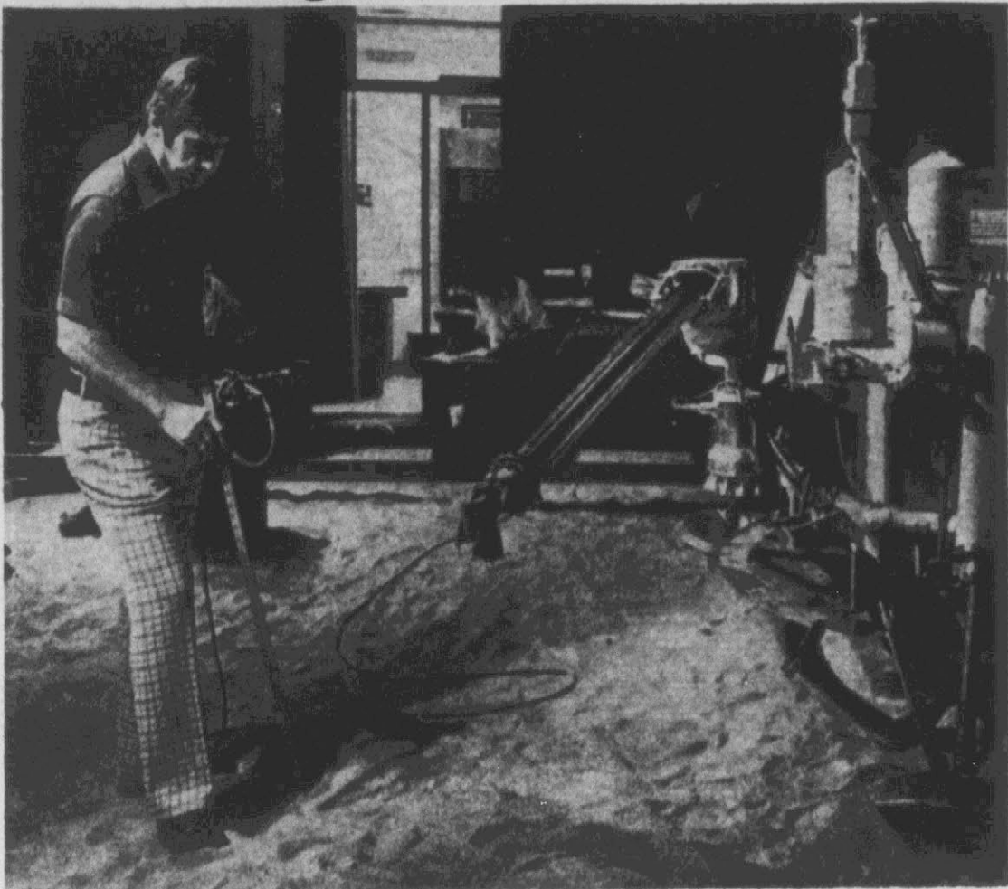
TESTING VIKING'S 'SICK' ARM—Using a working model of the Viking 1 lander at the Jet Propulsion Lab in Pasadena, Don Crouch, of the Viking Surface Sampler Team, works at pre-programming the Viking soil-scooping arm, which has become stuck. He's using a
