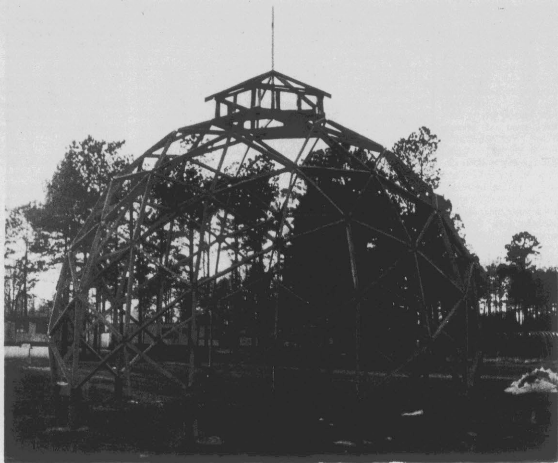
FRAME FINISHED . . . with the covering yet undone, reveals the basic framework of the geodesic dome the Lassiters built.
