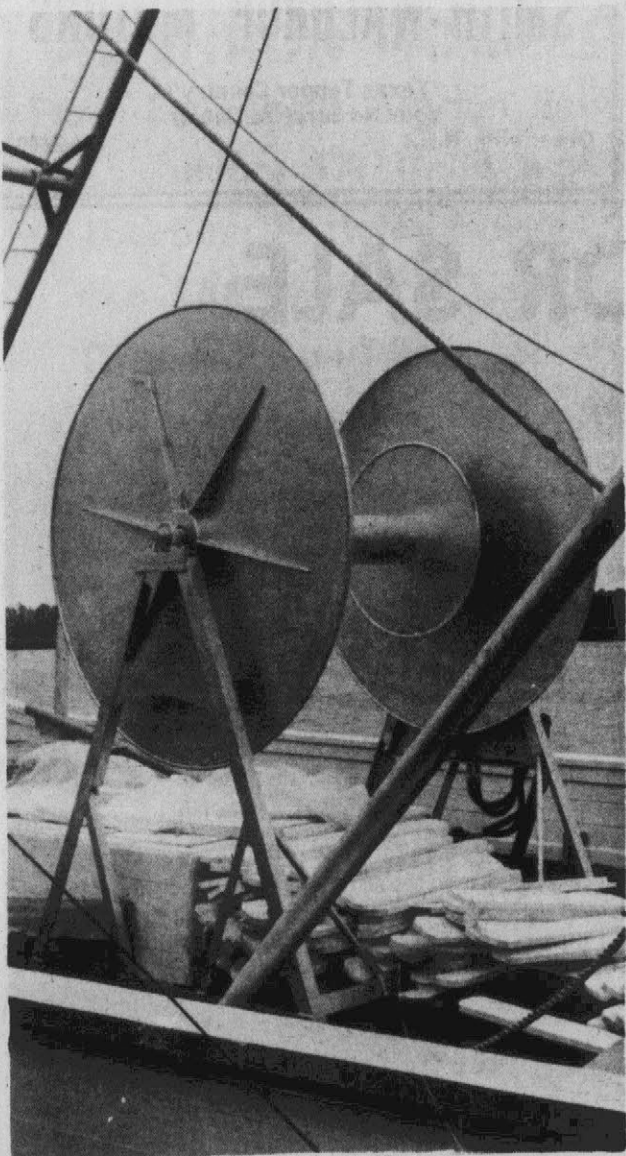
A LARGE NET WENCH . . . on the deck of "Lady Barbara" is designed for hauling in nets during deep-sea stern fishing.
