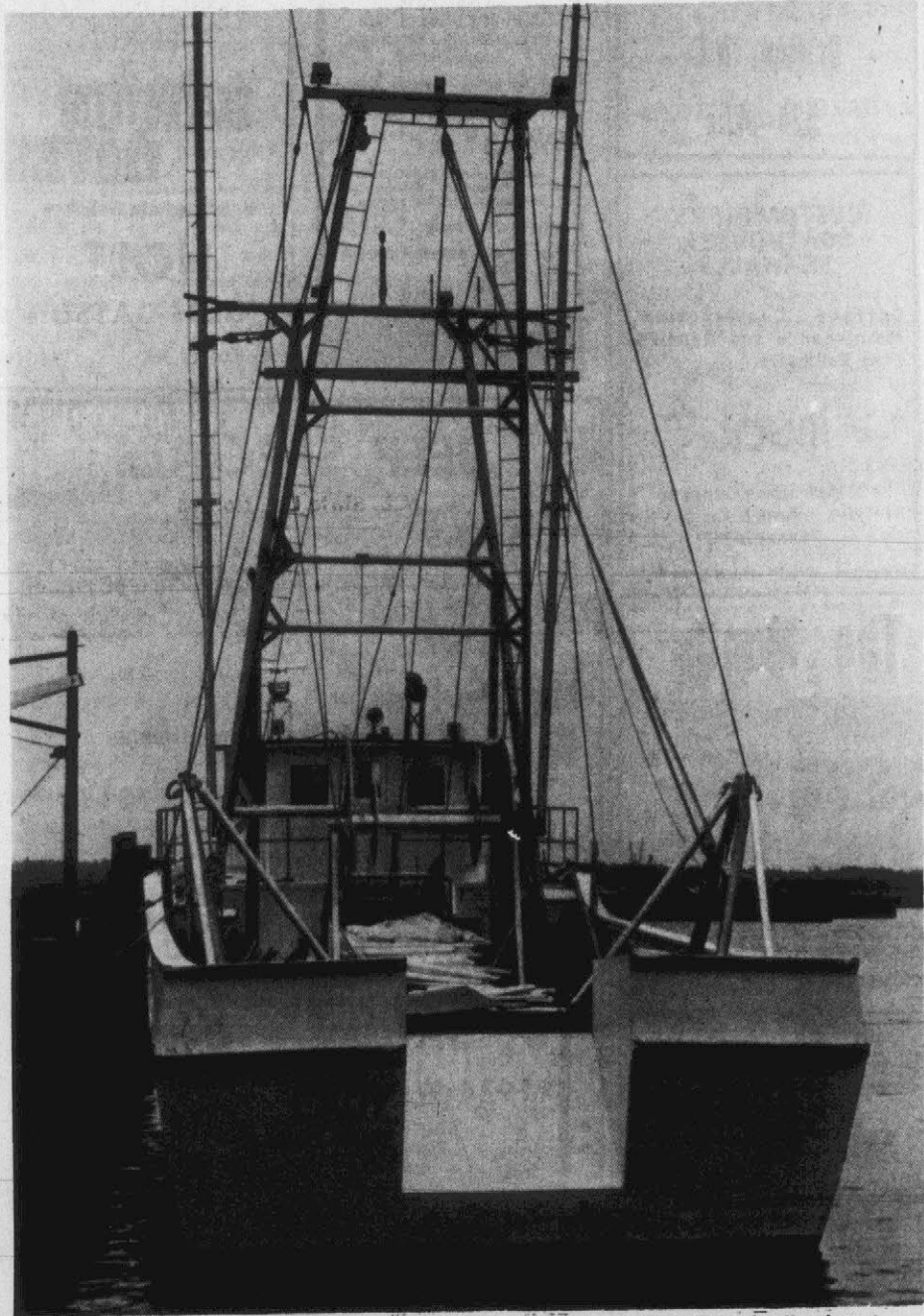
BACK VIEW . . . of the "Lady Barbara" reveals a stern ramp that will facilitate hauling in nets
